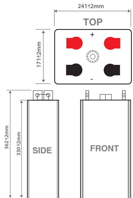
UXL550-2 GEN2 Battery Drawing
