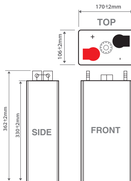
UXL220-2 GEN2 Battery Drawing
